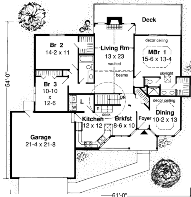
Slab/Crawl Space Option
